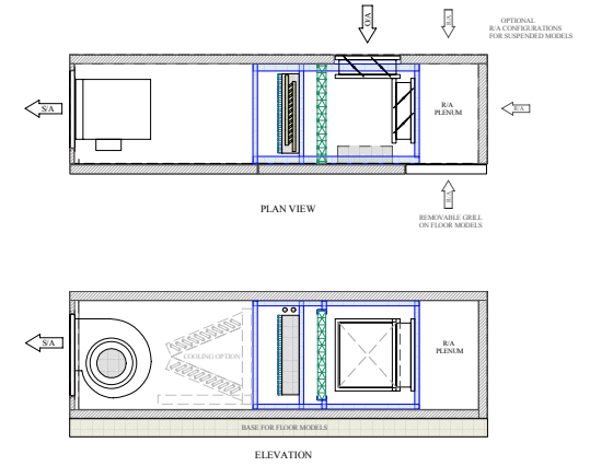
HORIZONTAL MODELS FLOOR MODEL / SUSPENDED MODEL - HW HEATING - CW / DX COOLING - OPTIONAL R/A CONFIGURATION - LEFT OR RIGHT DISCHARGE - AVAILABLE IN 1200, 1600, 2000 SIZES
