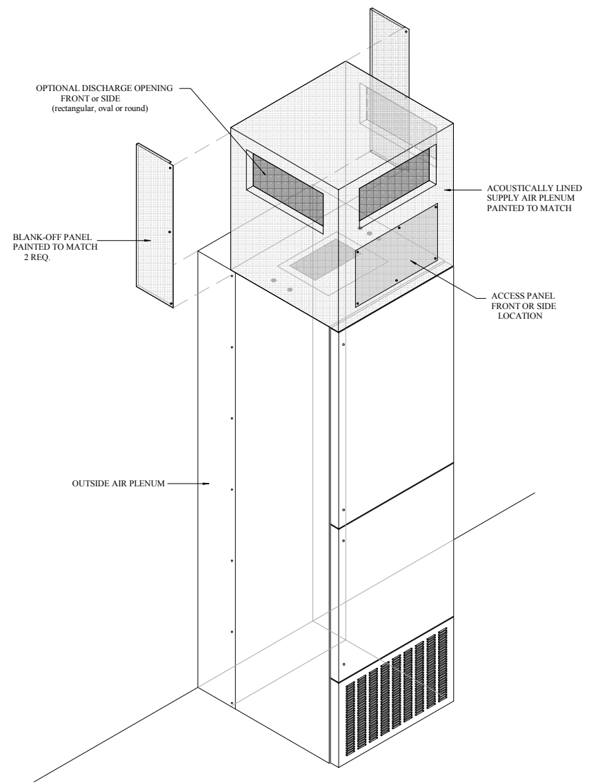
CENTRAL INSTALLATION
