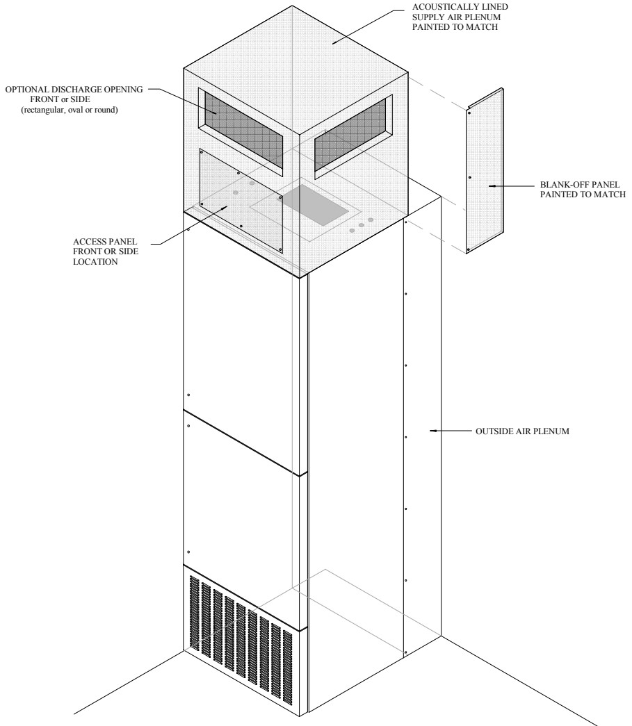
LEFT CORNER INSTALLATION
