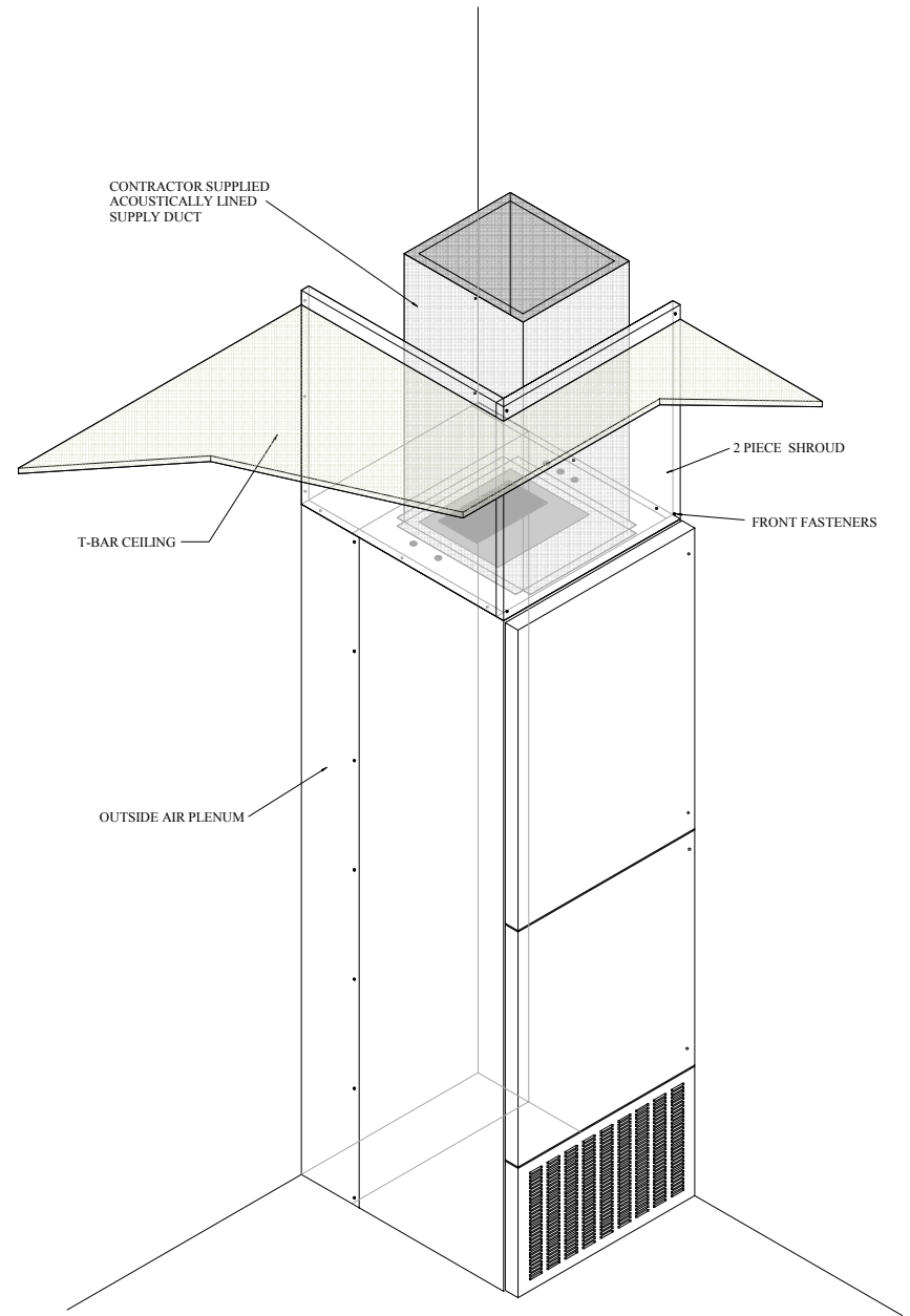
RIGHT CORNER INSTALLATION 2 PC. SHROUD
