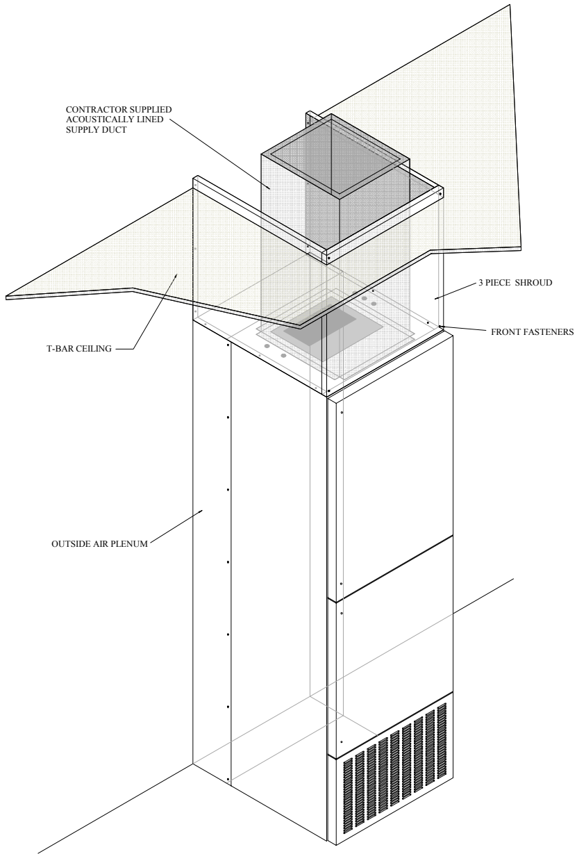
CENTRAL INSTALLATION 3 PC. SHROUD
